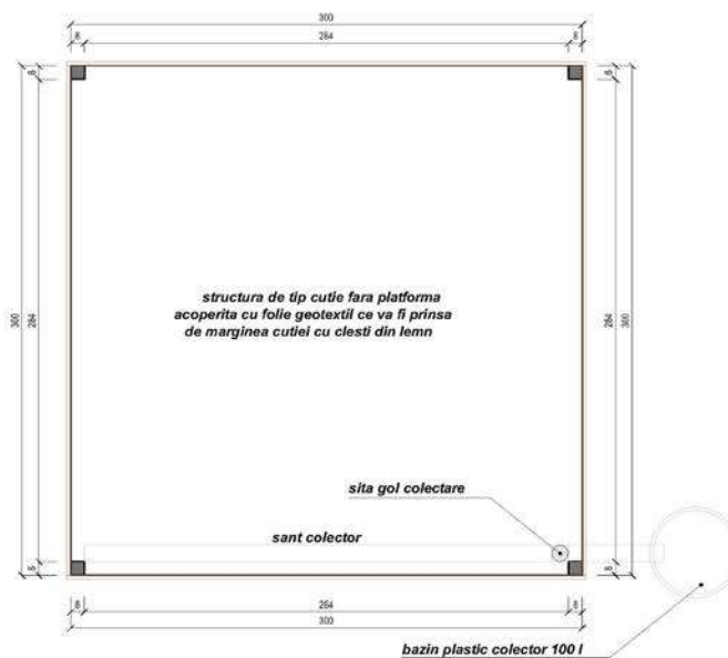
PLAN SC. 1:25
